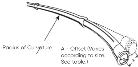
MAXIMUM RECOMMENDED OFFSET, A, TO ACHIEVE MINIMUM RADII OF CURVATURE BY BENDING THE BARREL OF 20 ft (6 m) LENGTHS
