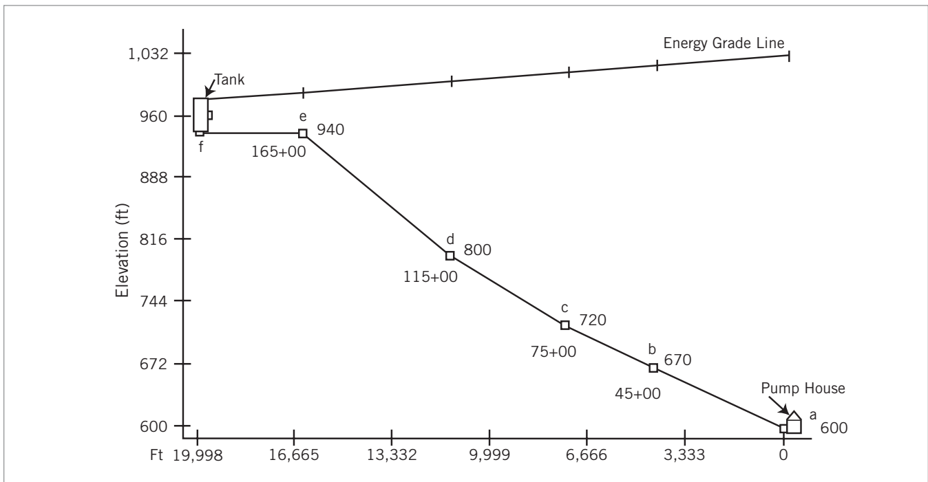
Figure 4 – Pipeline Profile
