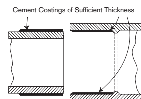
Figure 2: Solvent Cement Coatings of Sufficient Thickness Applied Uniformly around Pipe and inside Fitting Socket
