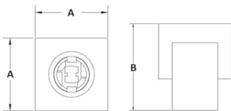
1/2" to 2"
